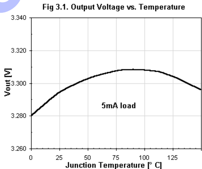
Fig 3.1. Output Voltage vs. Temperature. This shows the regulator V_{OUT} performance up to the maximum rated junction temperature. The overall 125°C variation in junction temperature causes an output voltage change of about 30mV.
