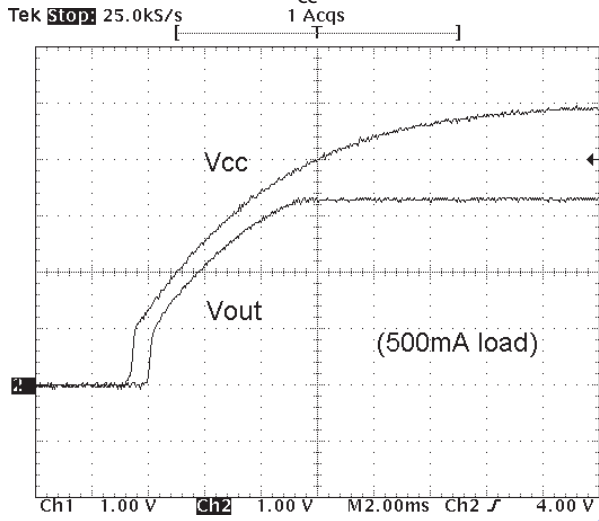
Fig 2.1 V_{CC} cold start
