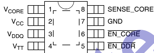
8-Lead PSOP
