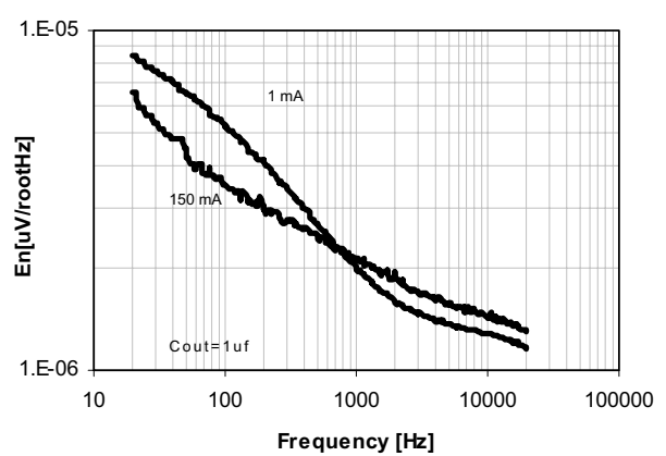
Output Noise (1uF Cout)
