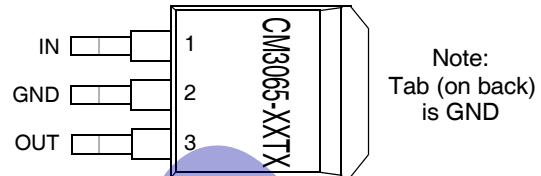
3-lead TO-263
