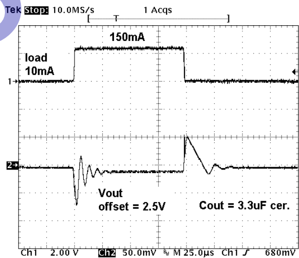
Figure 3. Stable Load Transient Response 2.5V output with 3.3µF ceramic capacitor
